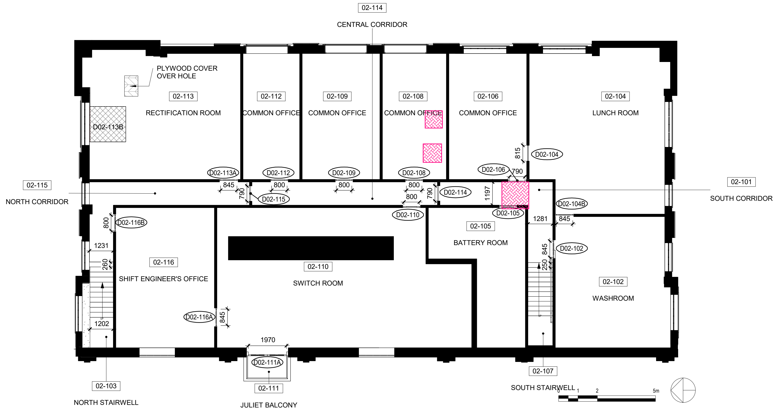
02 - SWITCH HOUSE REFLECTED CEILING PLAN 1 : 100
