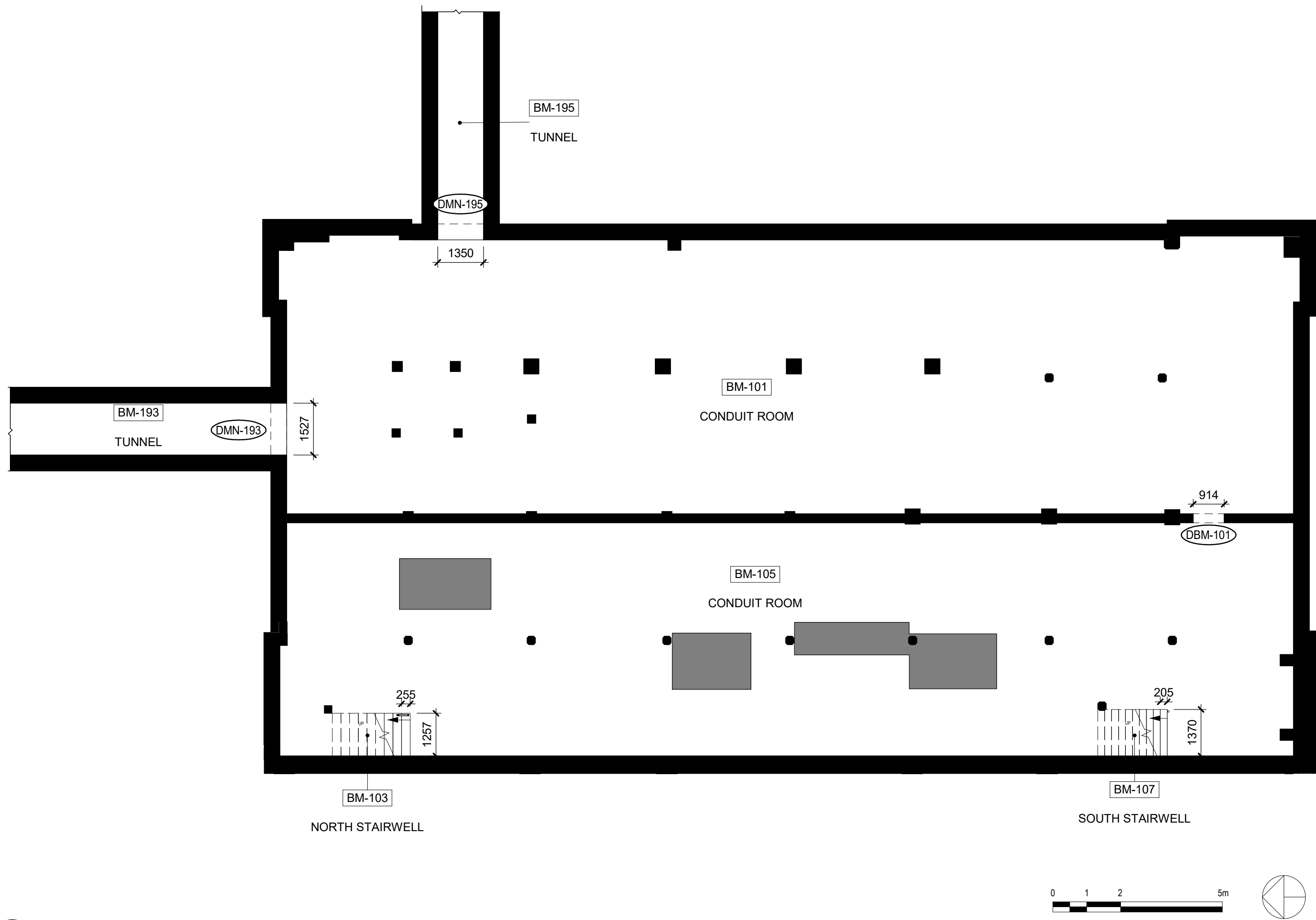
1 BM - SWITCH HOUSE REFLECTED CEILING PLAN 1 : 100
