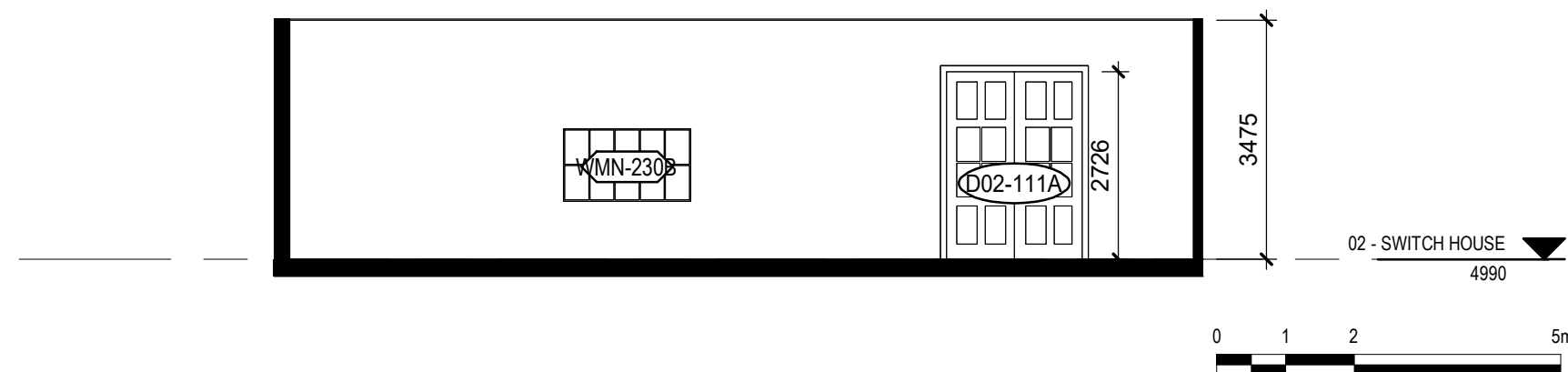
4 02 - SWITCH ROOM - WEST ELEVATION - SWITCH HOUSE 1 : 100
