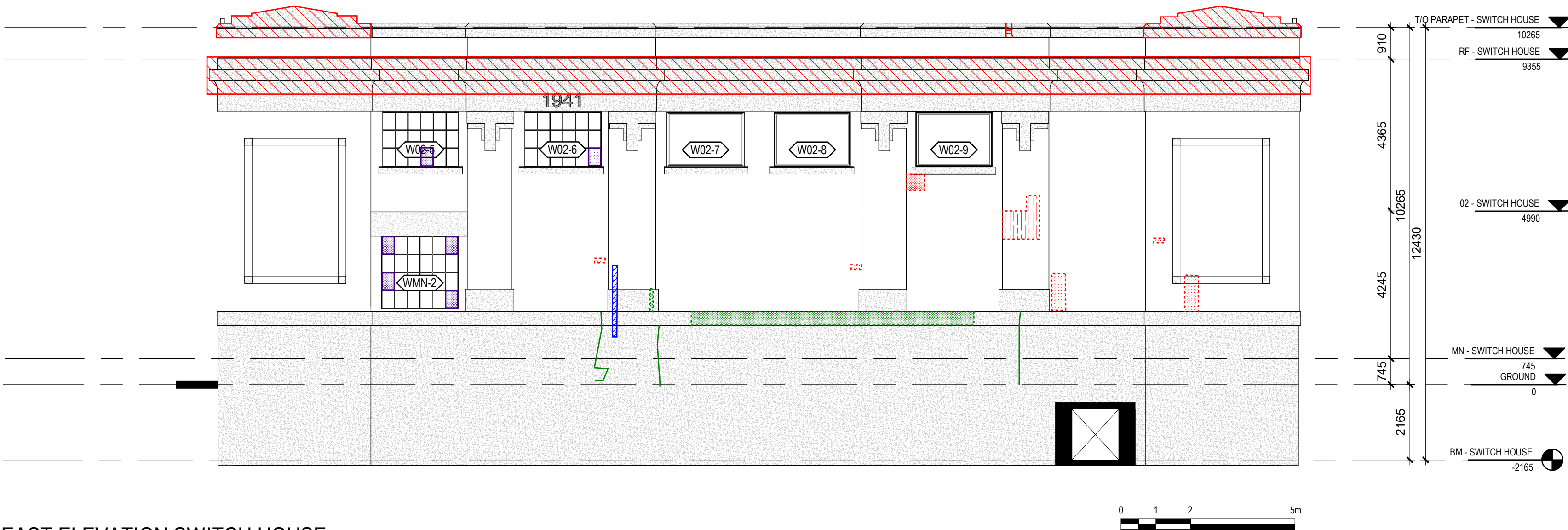
2 EAST ELEVATION SWITCH HOUSE 1 : 100
