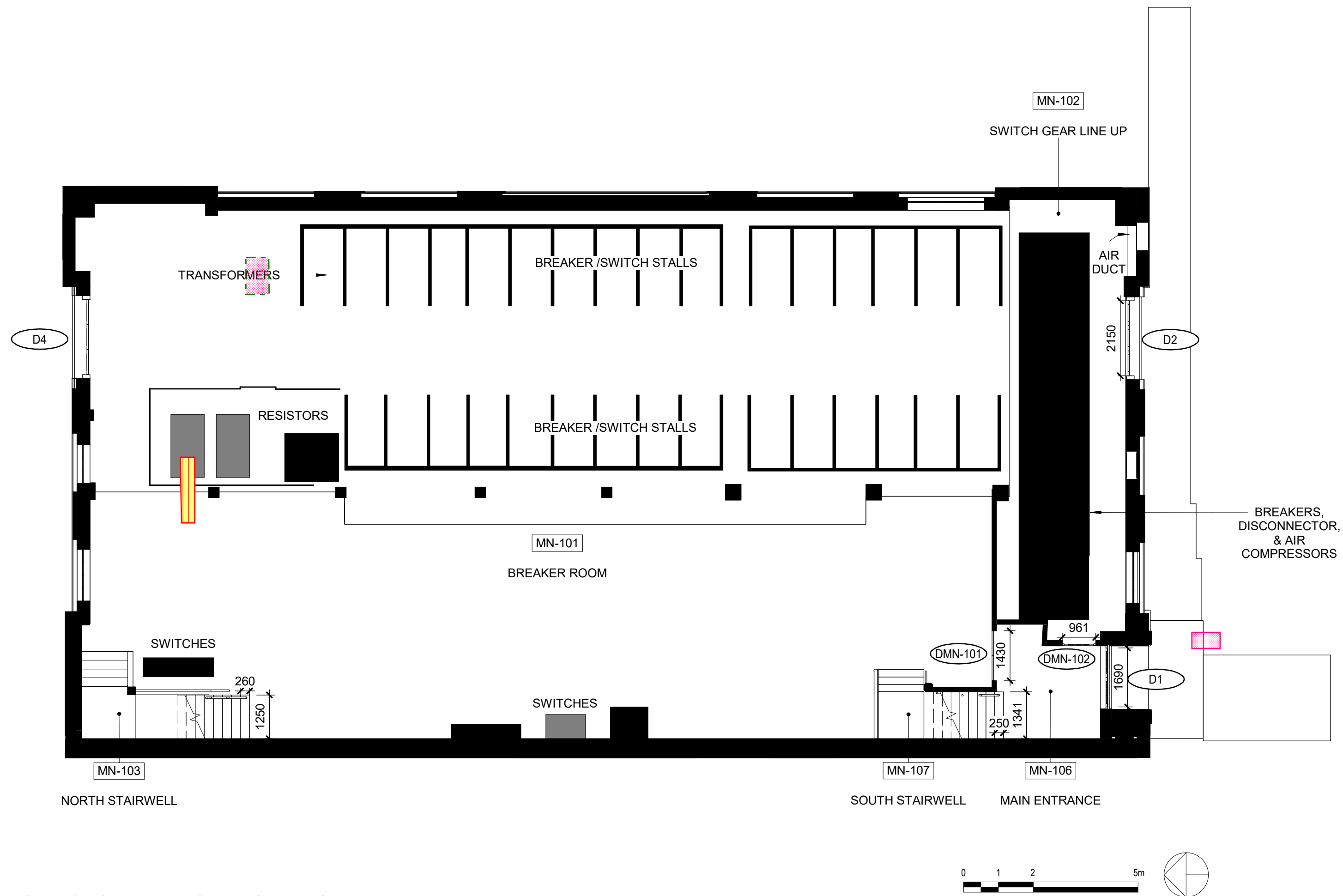
2 MN - SWITCH HOUSE REFLECTED CEILING PLAN 1 : 100
