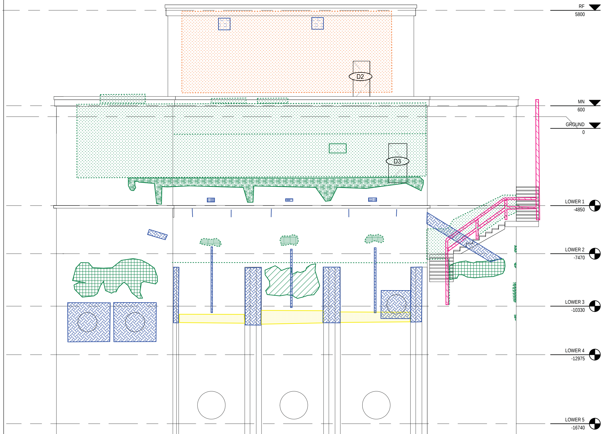
3 SOUTH ELEVATION 1 : 100
