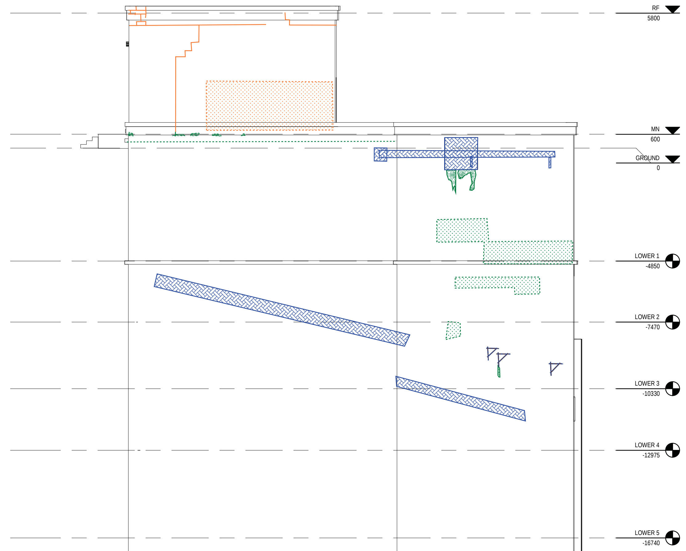
4 WEST ELEVATION 1 : 100
