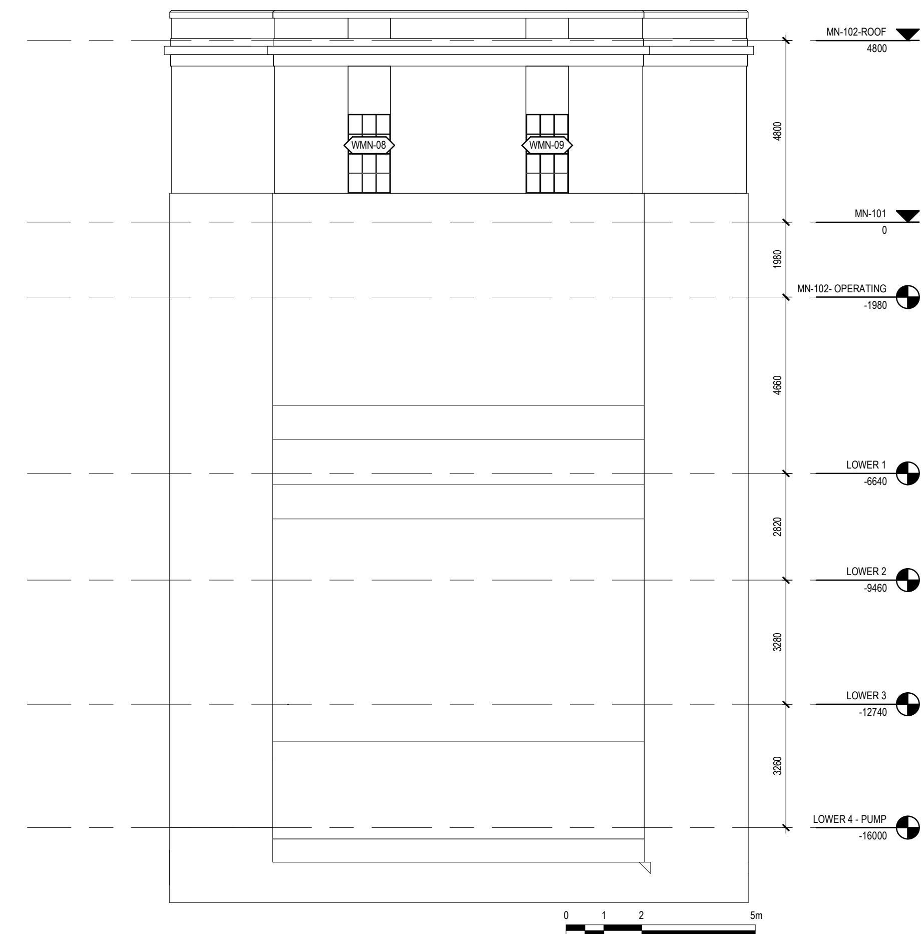
3 ELEVATION SOUTH 1 : 100
