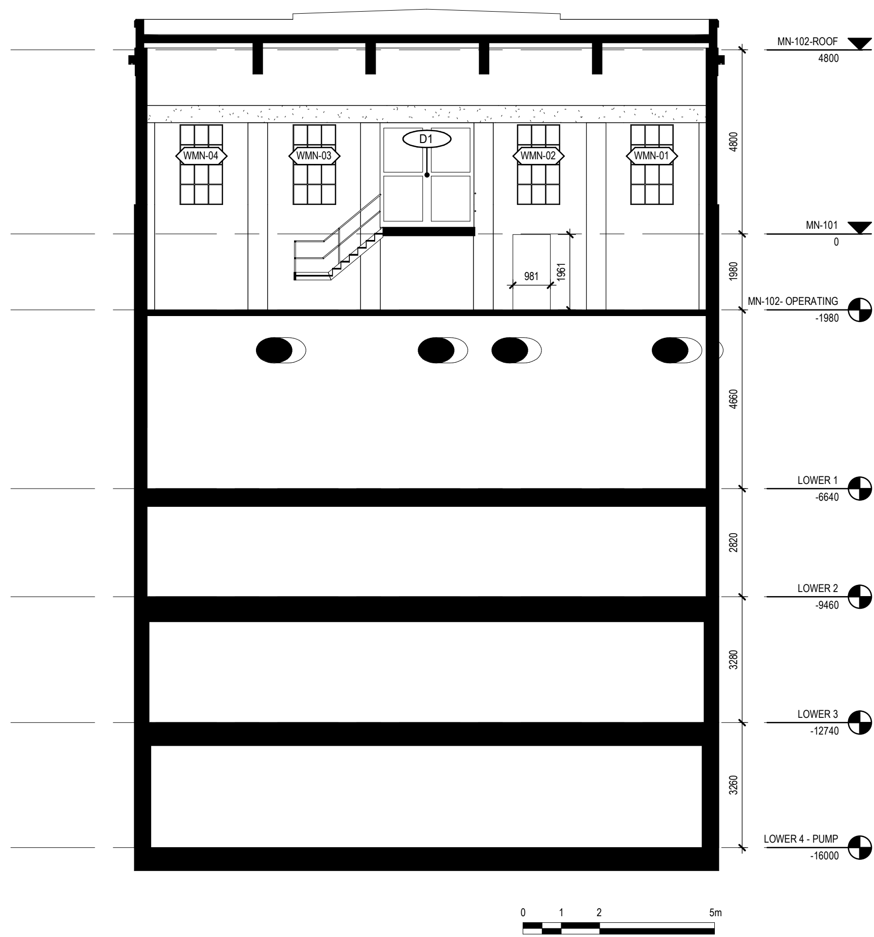
1 INTERIOR NORTH 1 : 100
