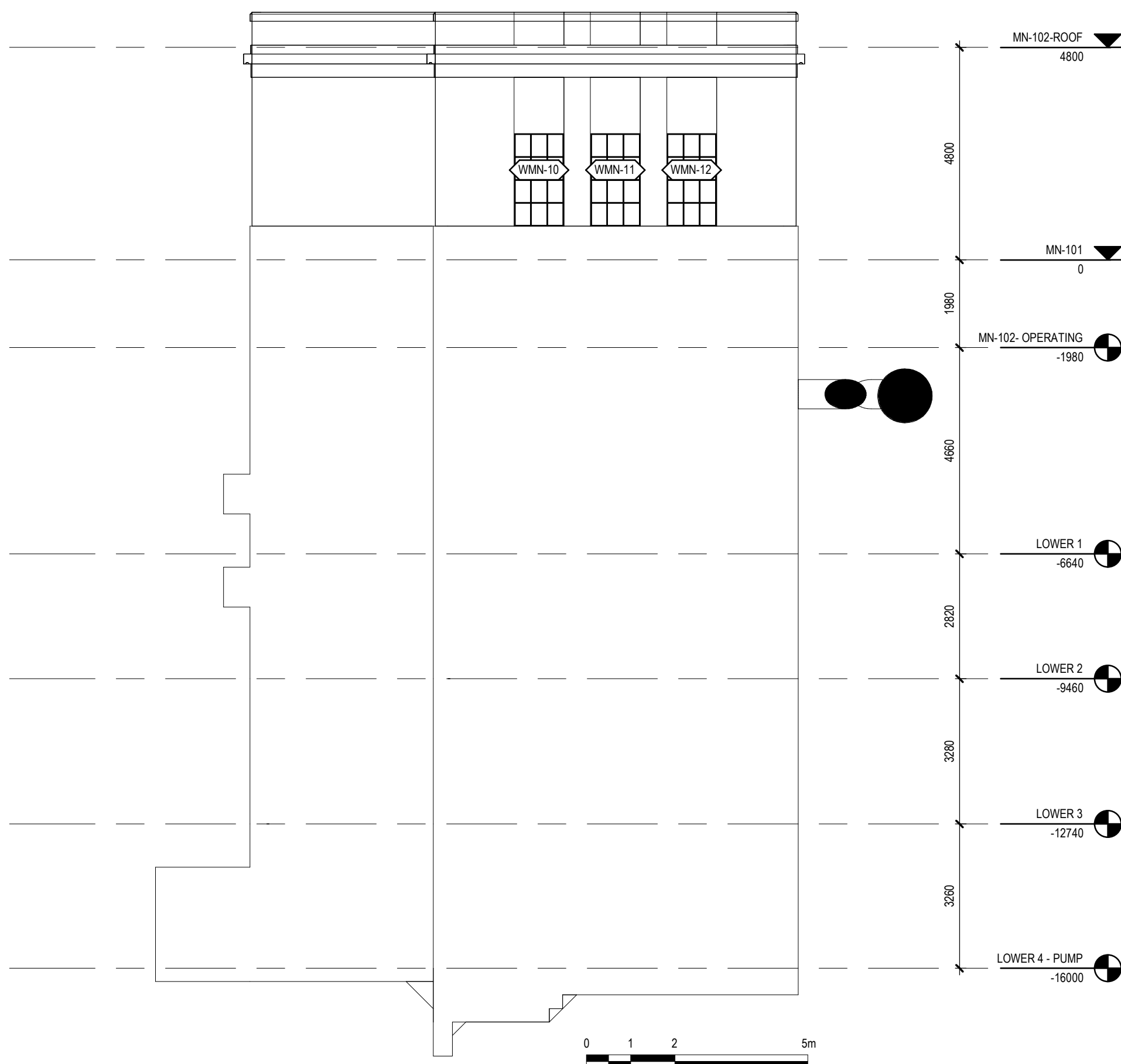
4 ELEVATION WEST 1 : 100
