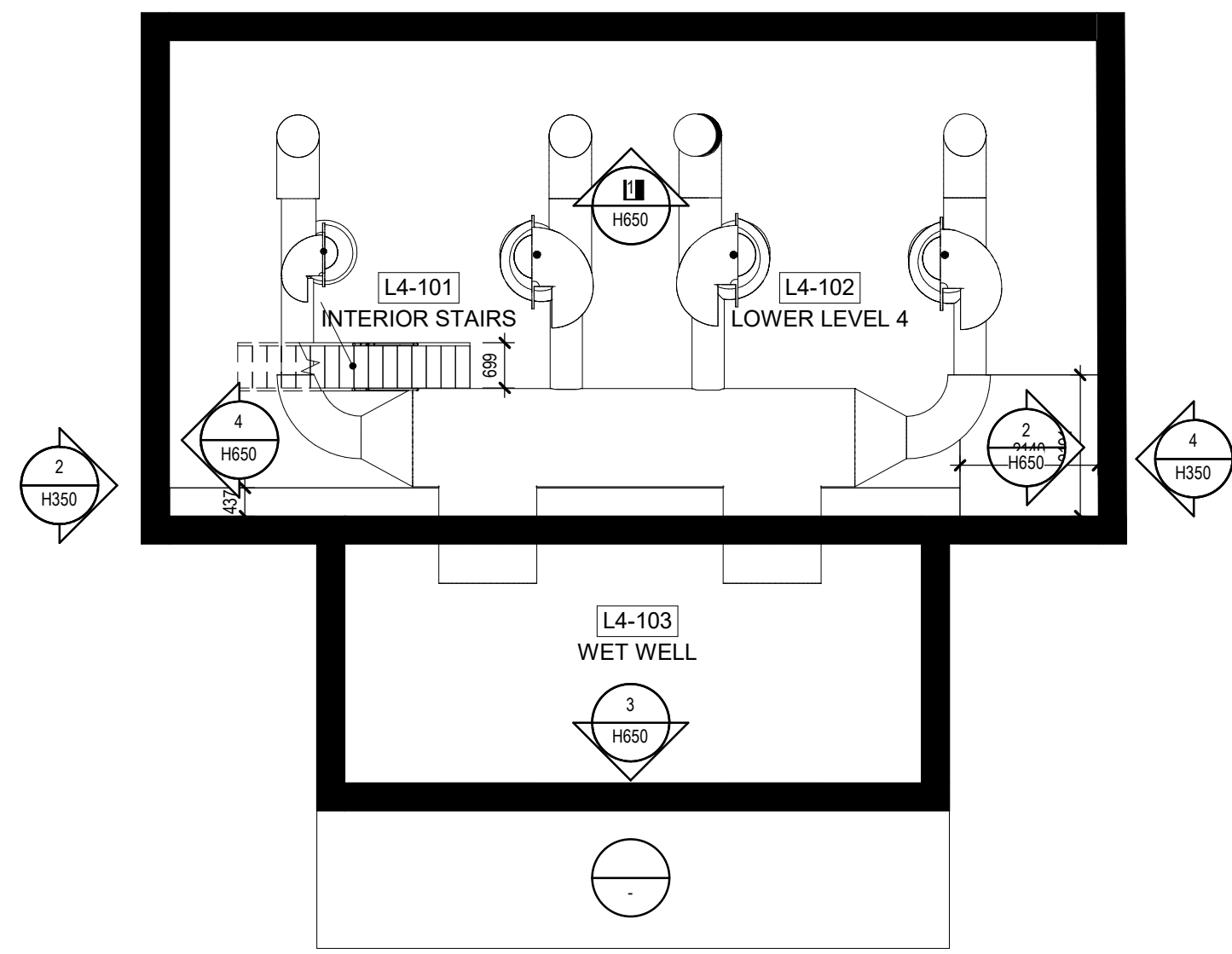
5 LOWER 4 - PUMP 1 : 100
