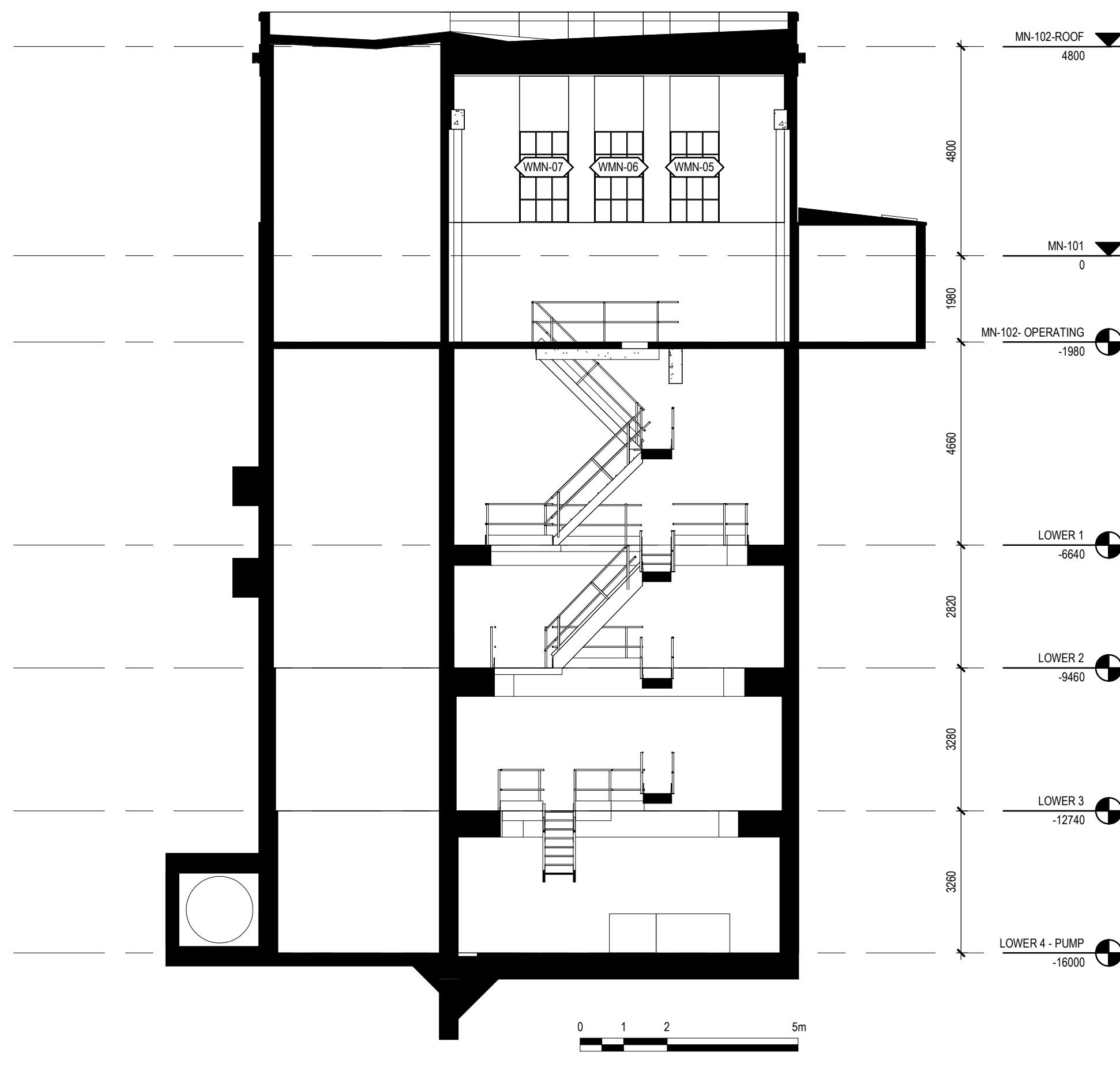
4 INTERIOR WEST 1 : 100
