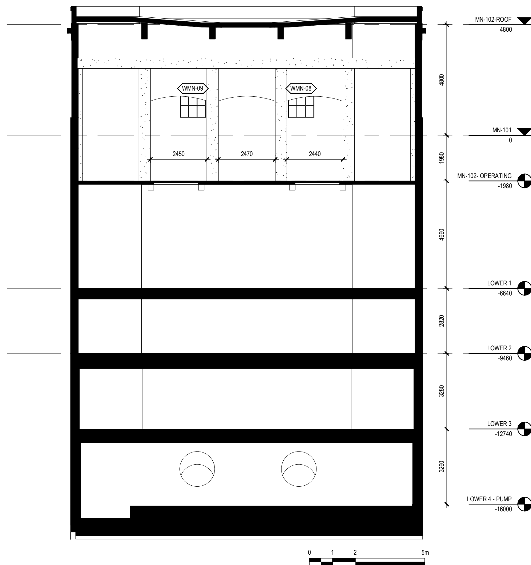
3 INTERIOR SOUTH 1 : 100
