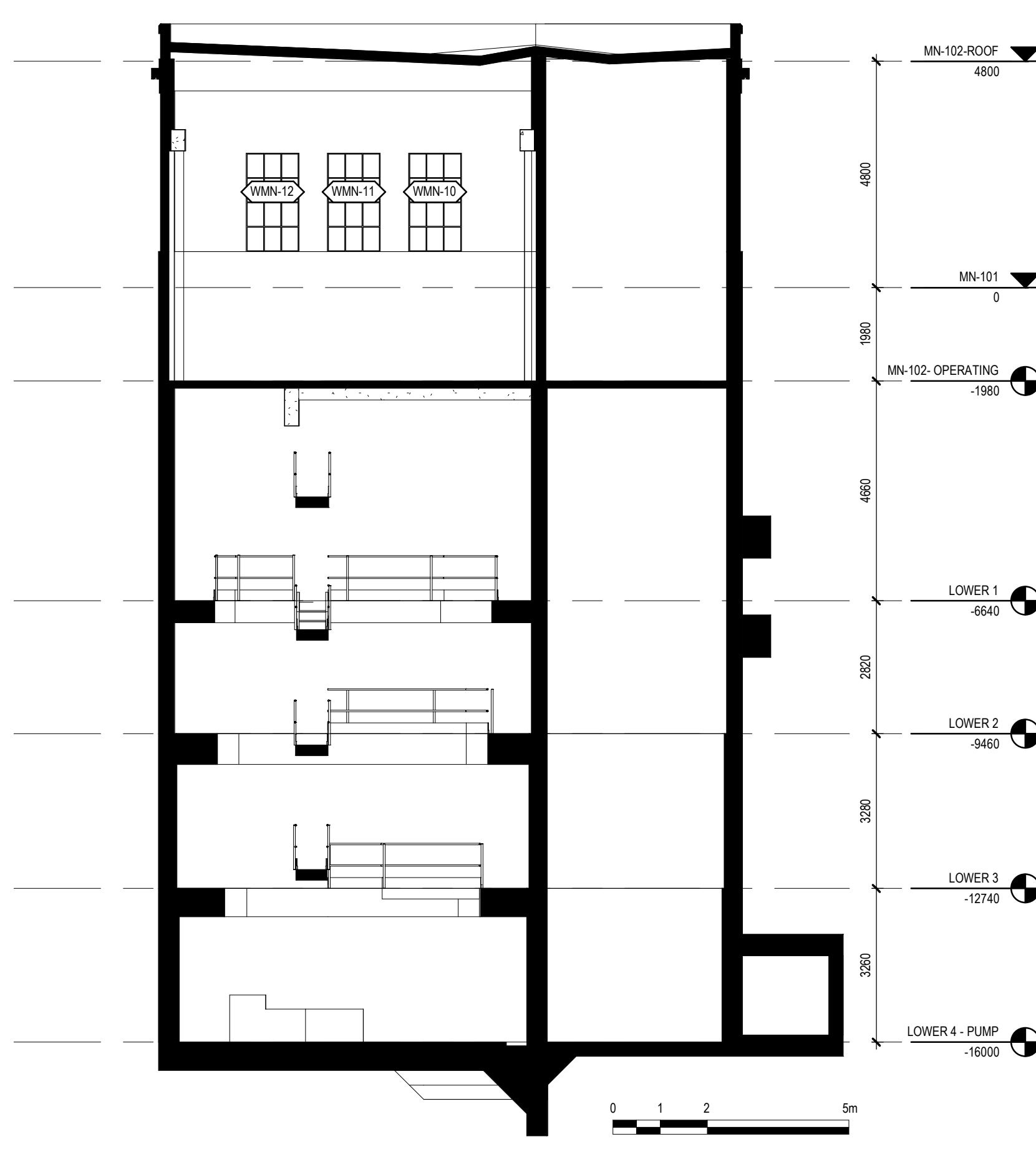
2 INTERIOR EAST 1 : 100
