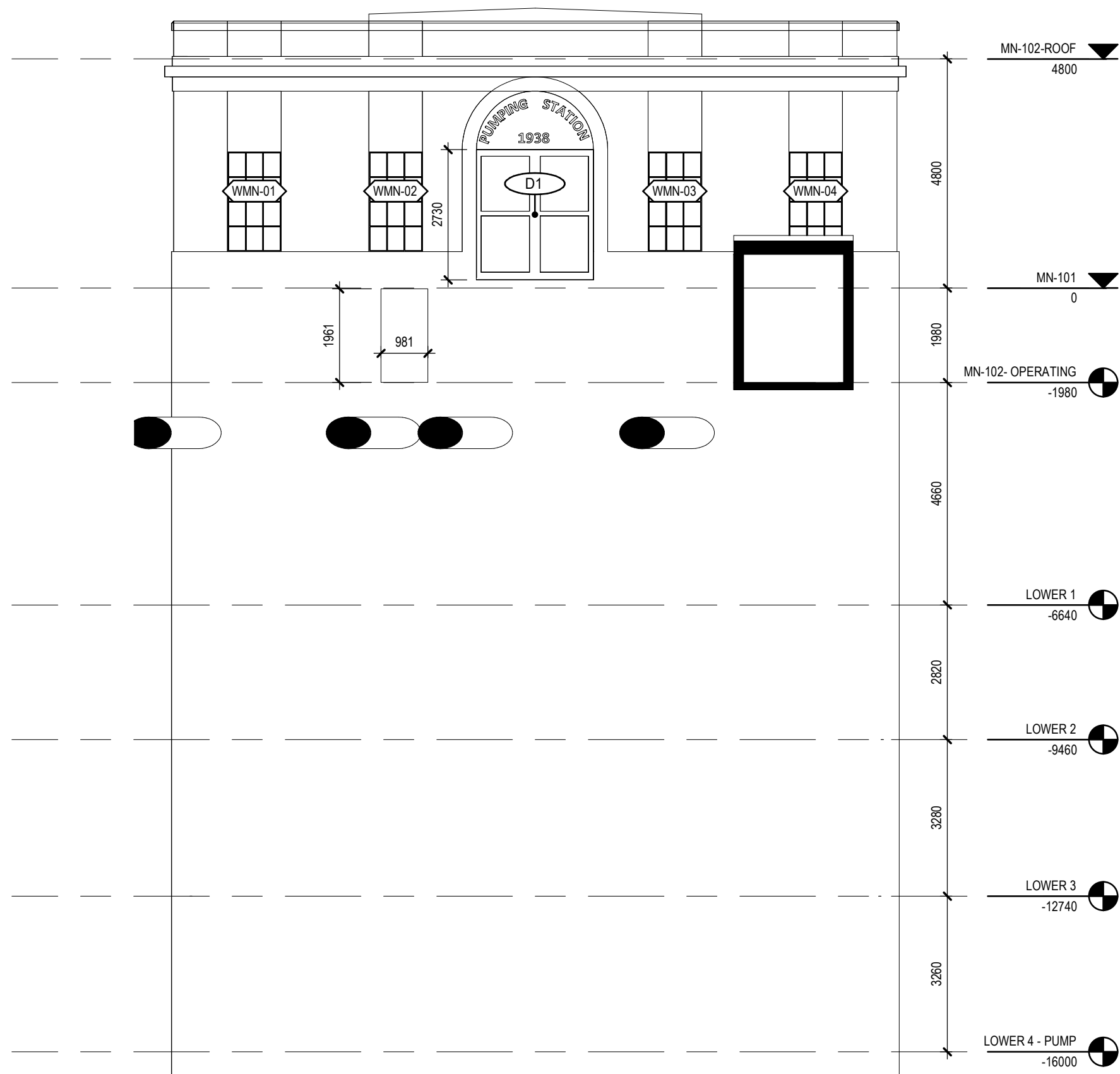
1 ELEVATION NORTH 1 : 100
