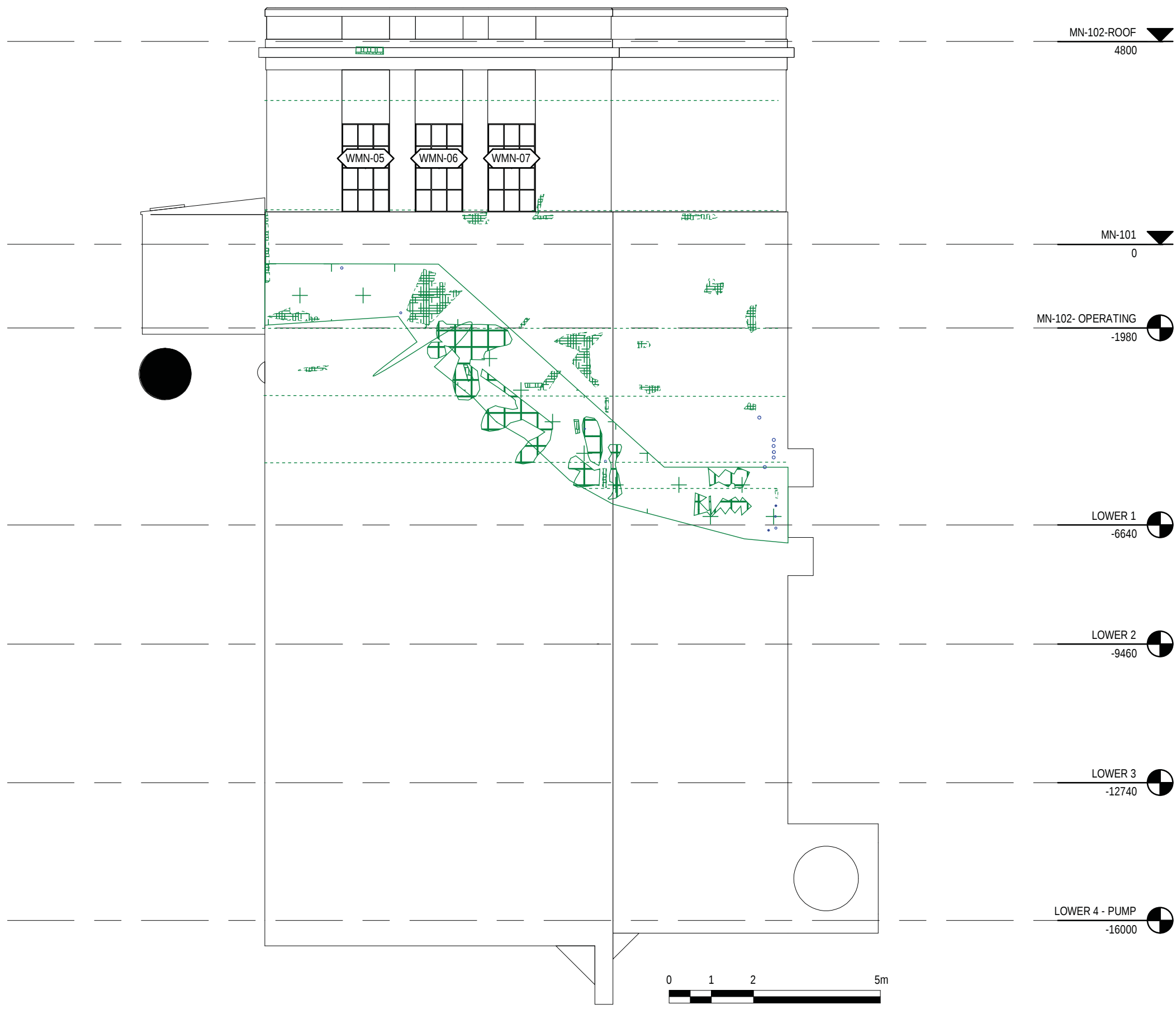
2 ELEVATION EAST 1 : 100
