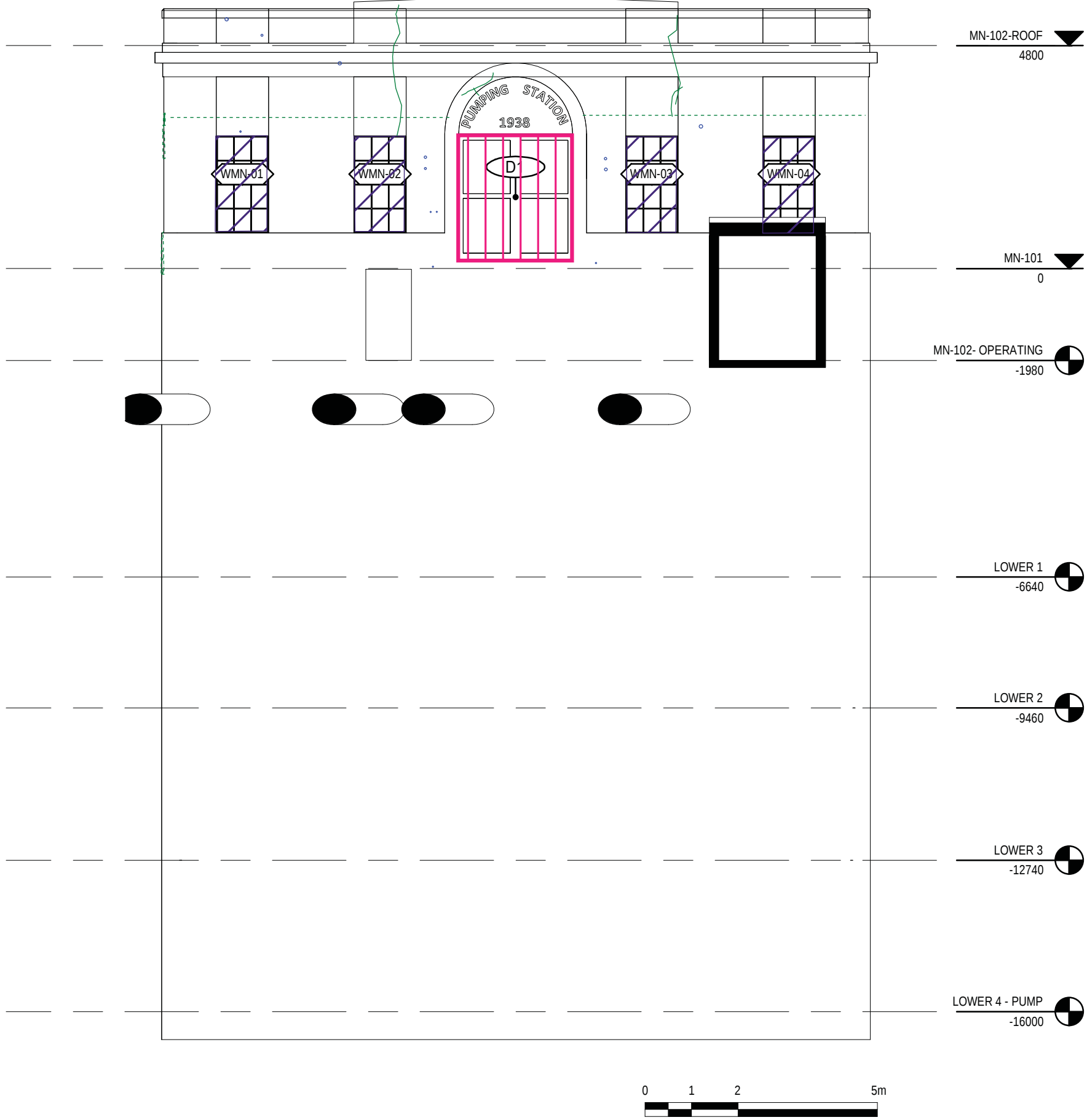
1 ELEVATION NORTH 1 : 100
