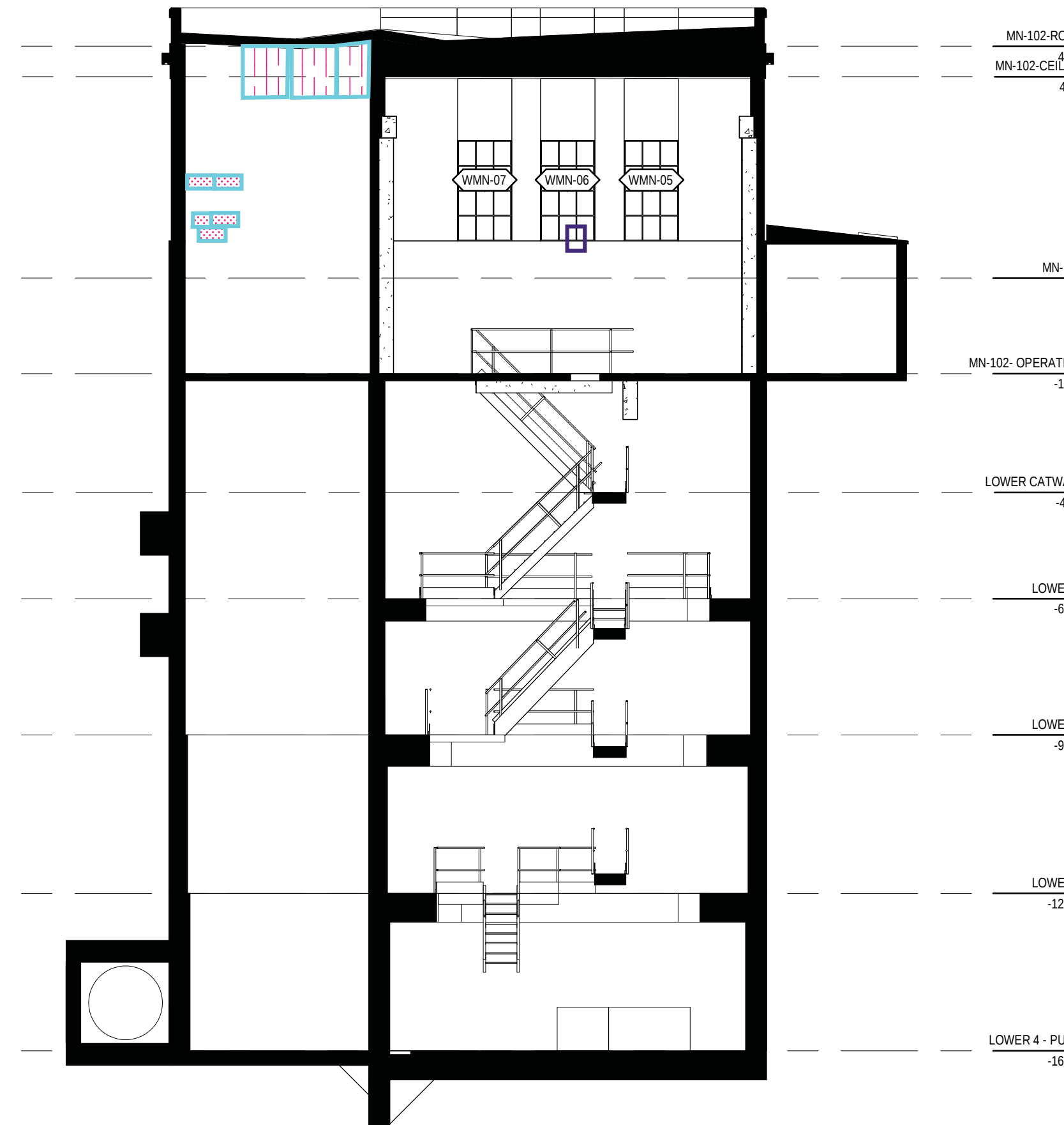
4 INTERIOR WEST 1 : 100
