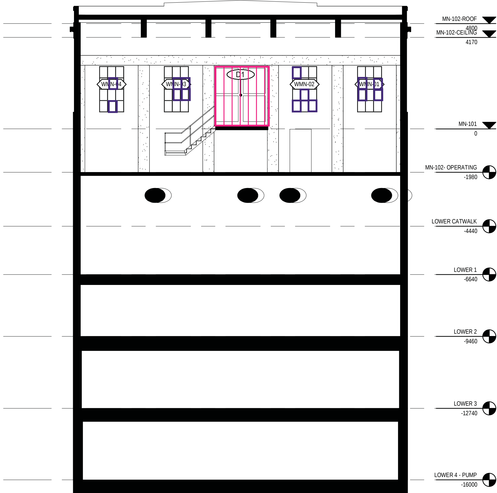
1 INTERIOR NORTH 1 : 100
