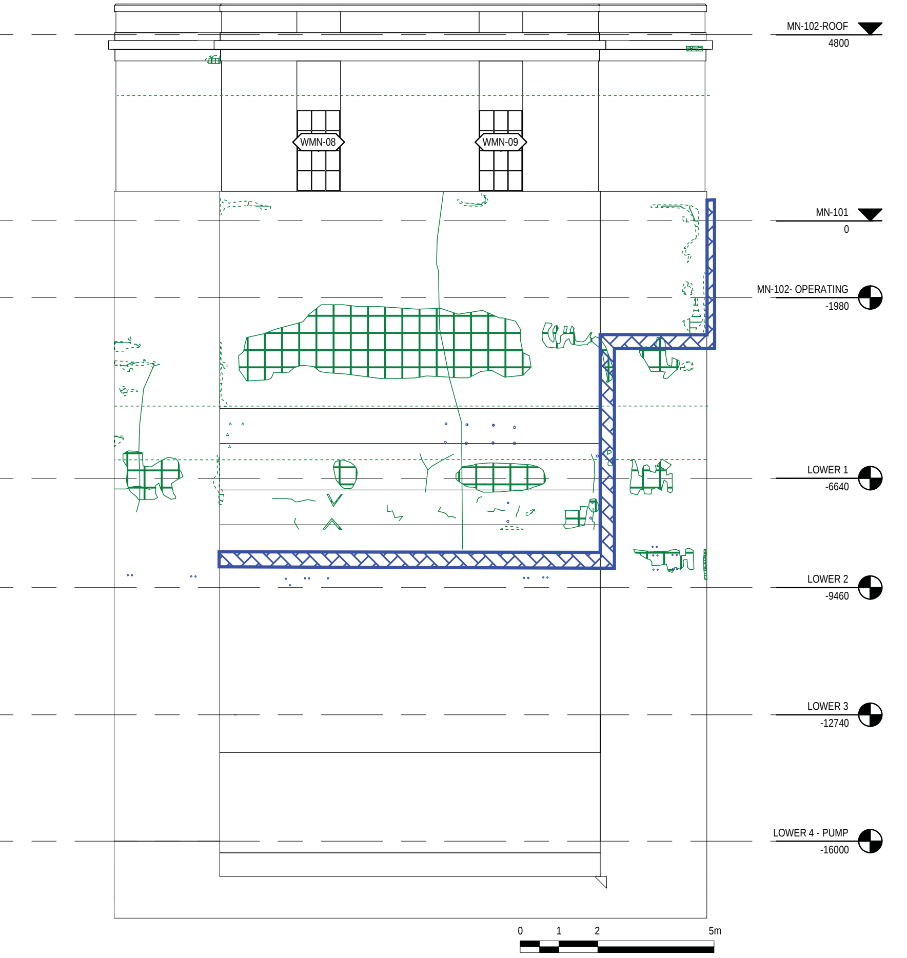
3 ELEVATION SOUTH 1 : 100
