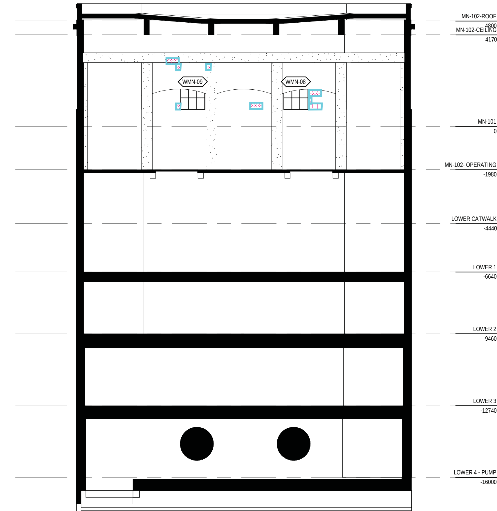
3 INTERIOR SOUTH 1 : 100
