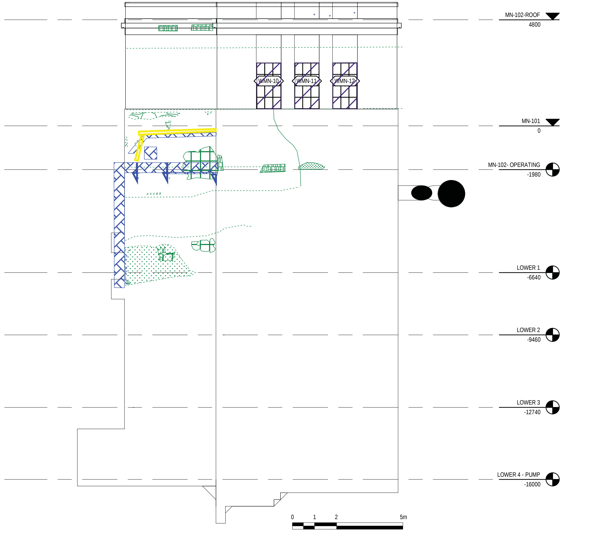
4 ELEVATION WEST 1 : 100
