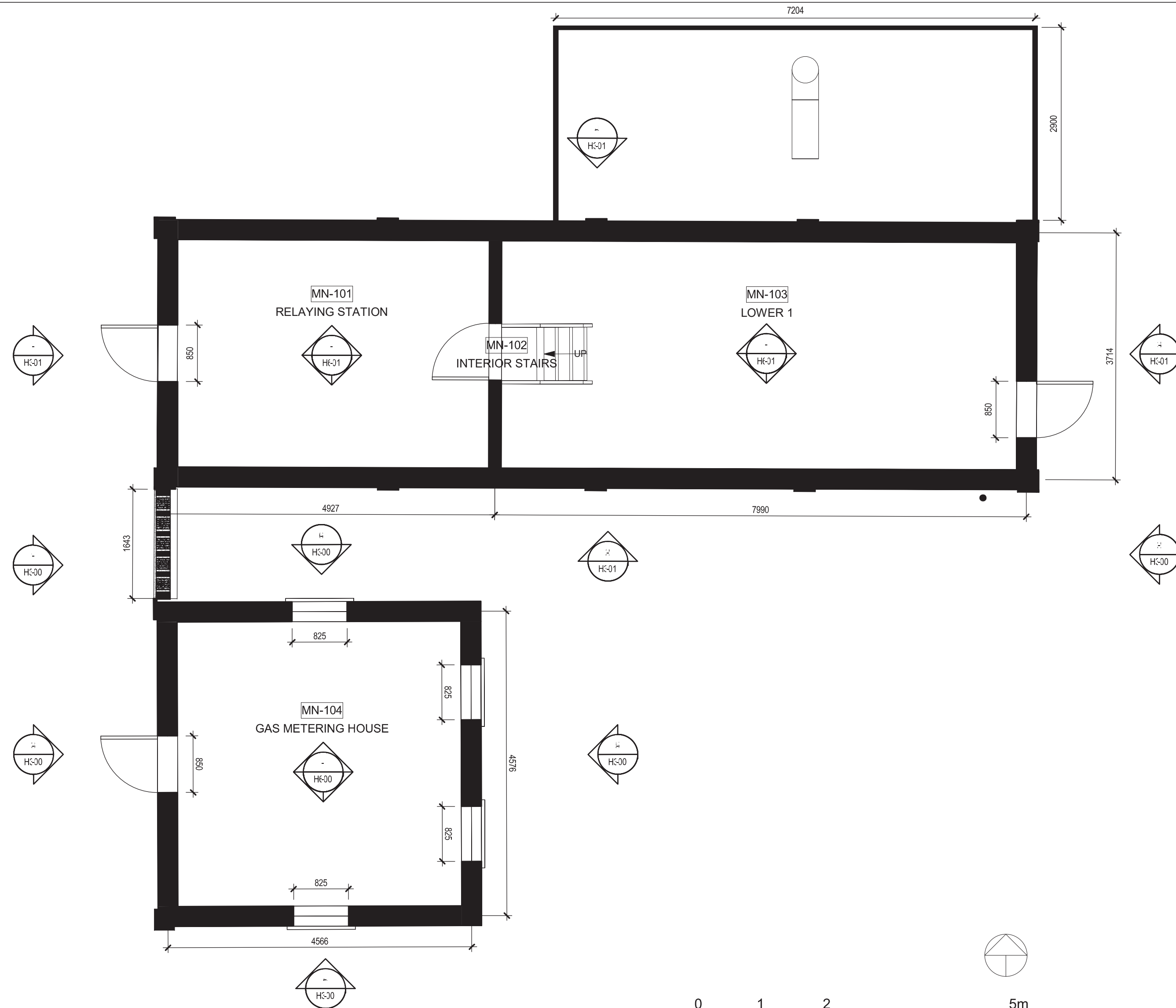
1 MAIN FLOOR 1 : 50
