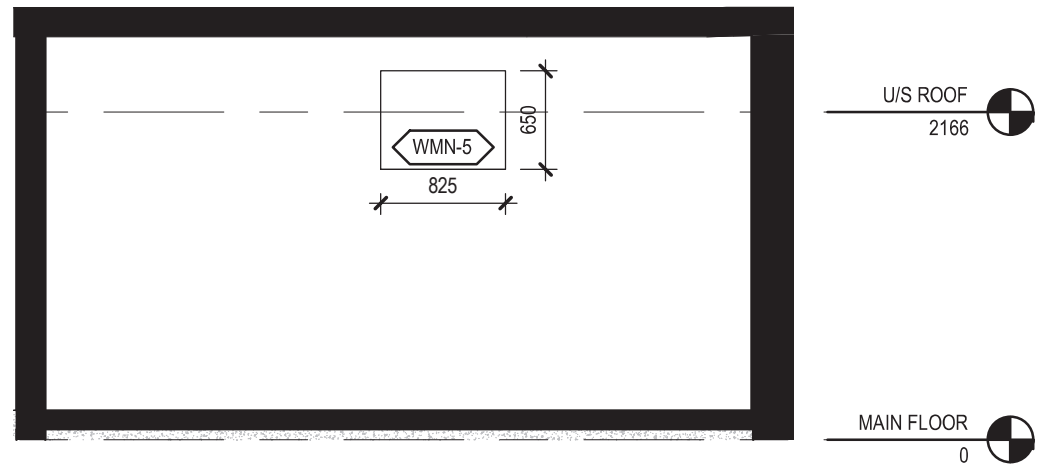
2 MN-101 INTERIOR SOUTH ELEVATION 1 : 50
