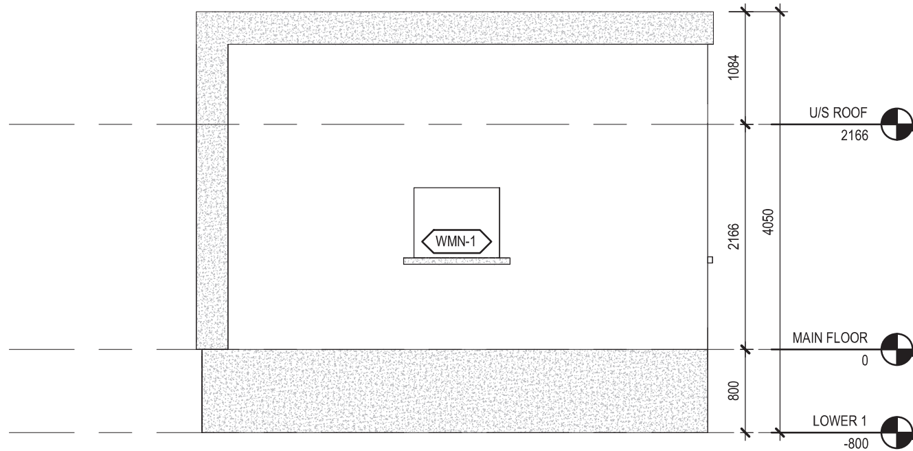
4 GAS METERING HOUSE SOUTH ELEVATION 1 : 50
