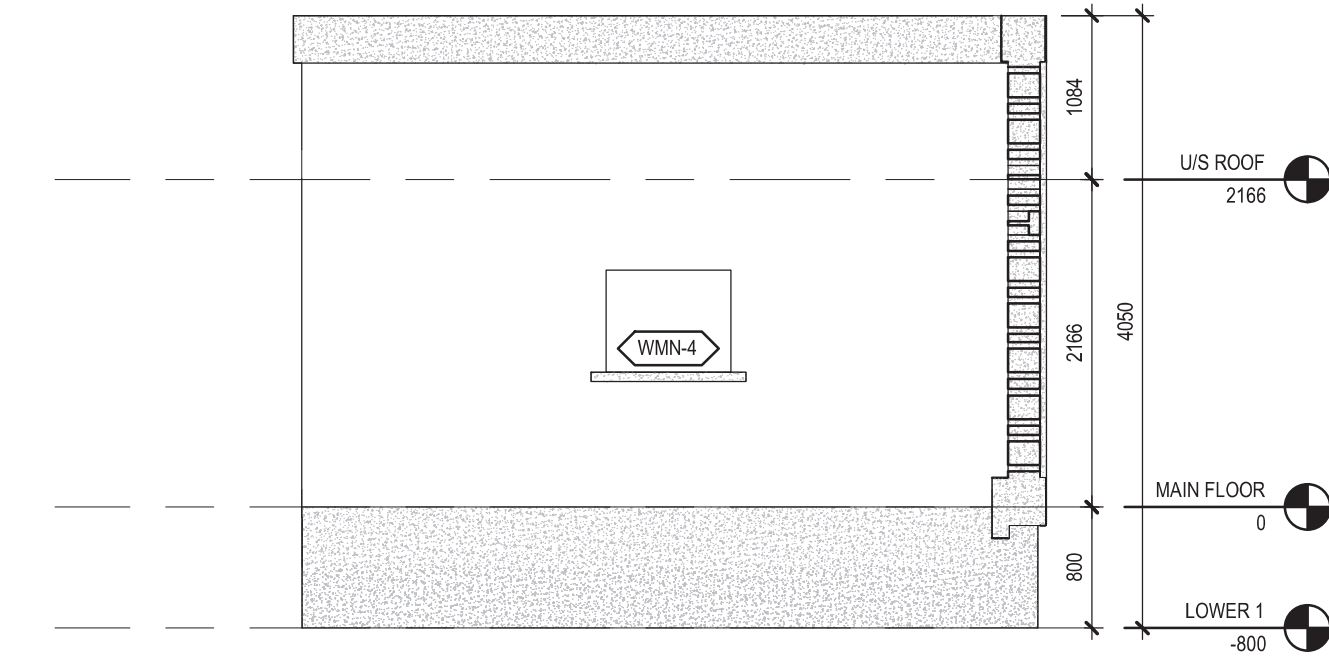
6 GAS METERING HOUSE NORTH ELEVATION 1 : 50
