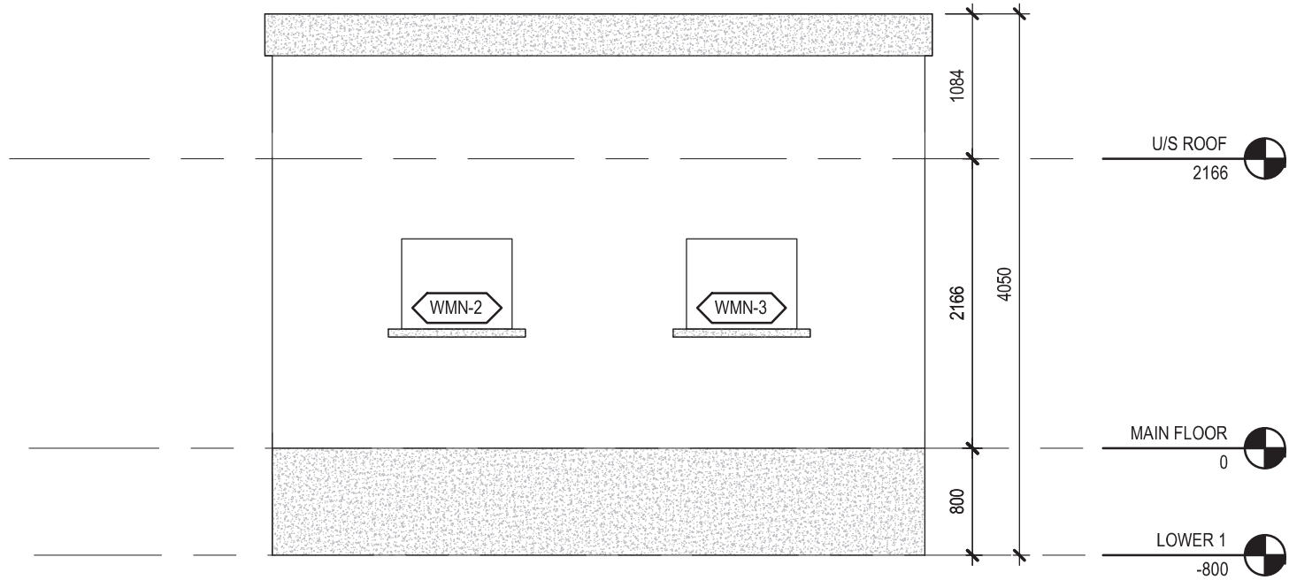
5 GAS METERING HOUSE EAST ELEVATION 1 : 50
