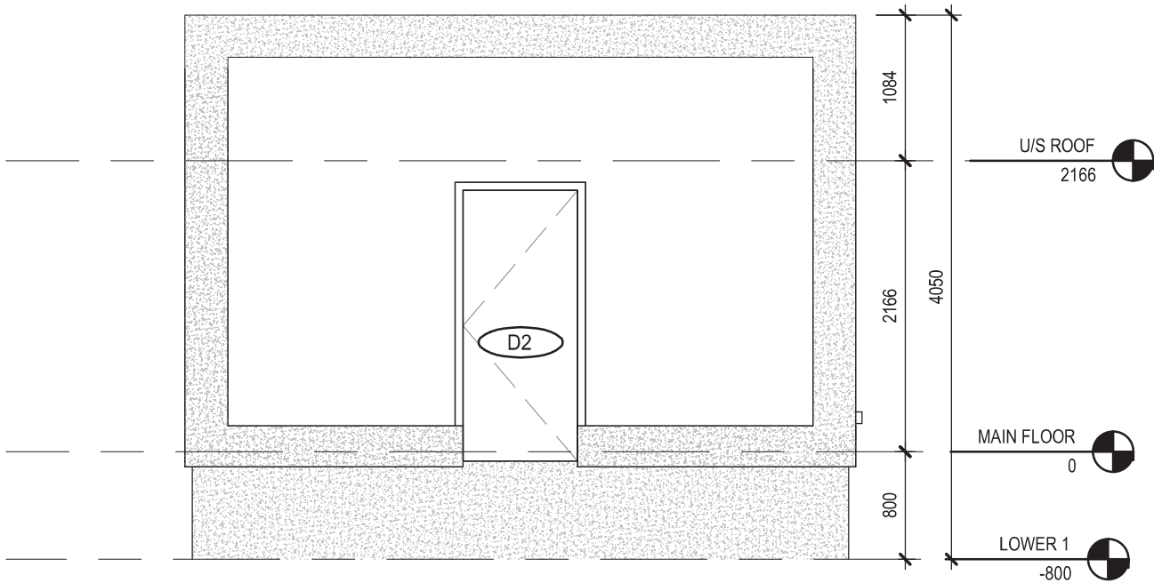
3 GAS METERING HOUSE WEST ELEVATION 1 : 50
