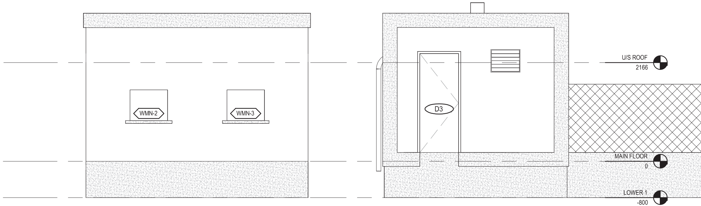
2 ATCO BUILDING EAST ELEVATION 1 : 50
