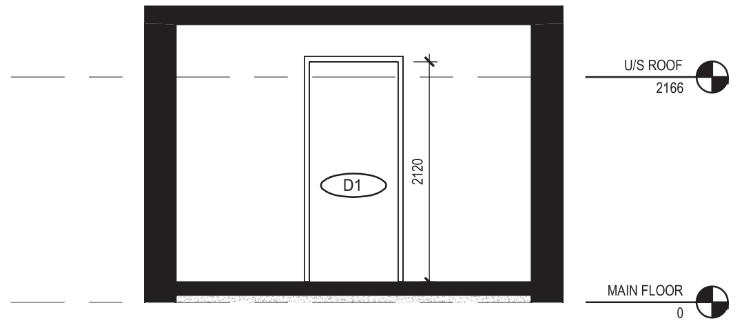
1 MN-101 INTERIOR WEST ELEVATION 1 : 50
