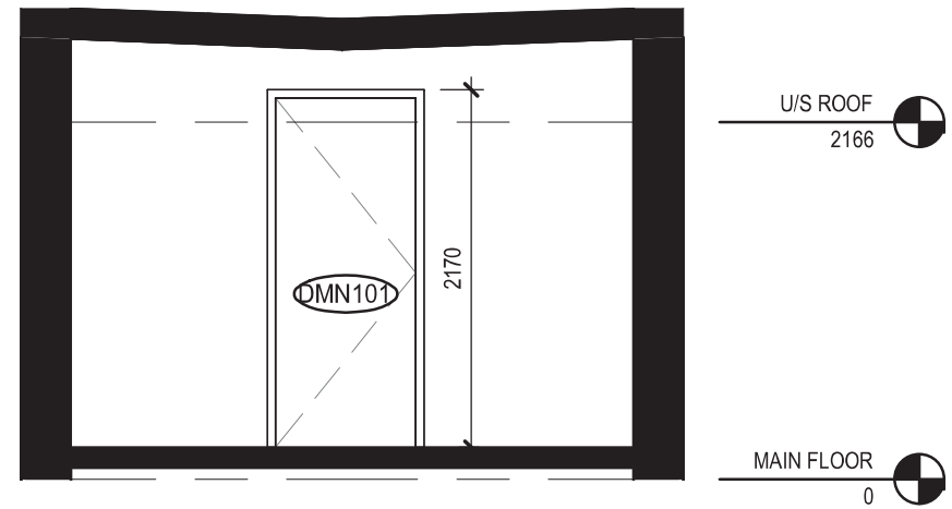
3 MN-101 INTERIOR EAST ELEVATION 1 : 50
