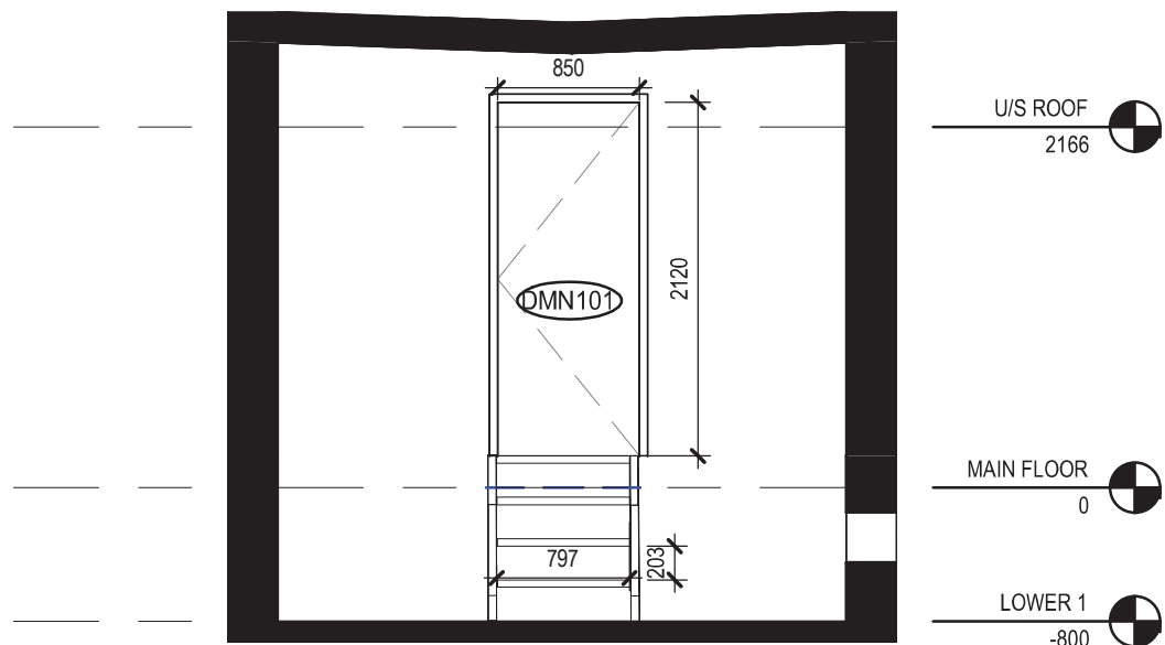
5 MN-103 INTERIOR WEST ELEVATION 1 : 50
