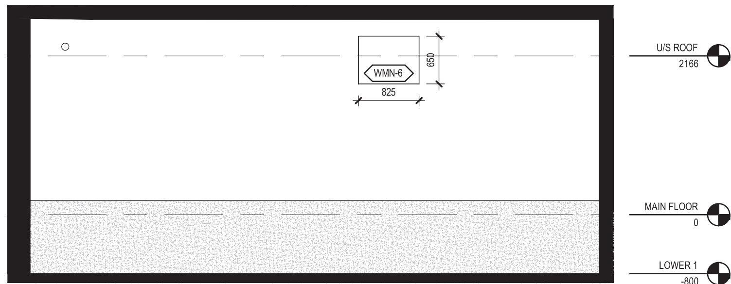
6 MN-103 INTERIOR SOUTH ELEVATION 1 : 50
