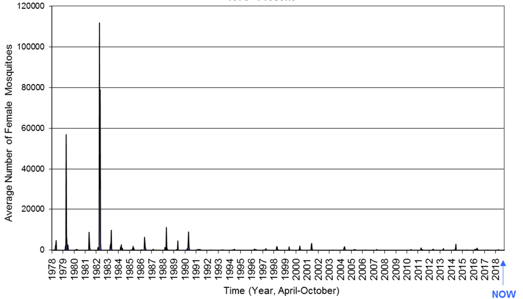
Average Weekly Light Trap Counts of Female Aedes Mosquitoes in the Edmonton Area 1978 - Present
