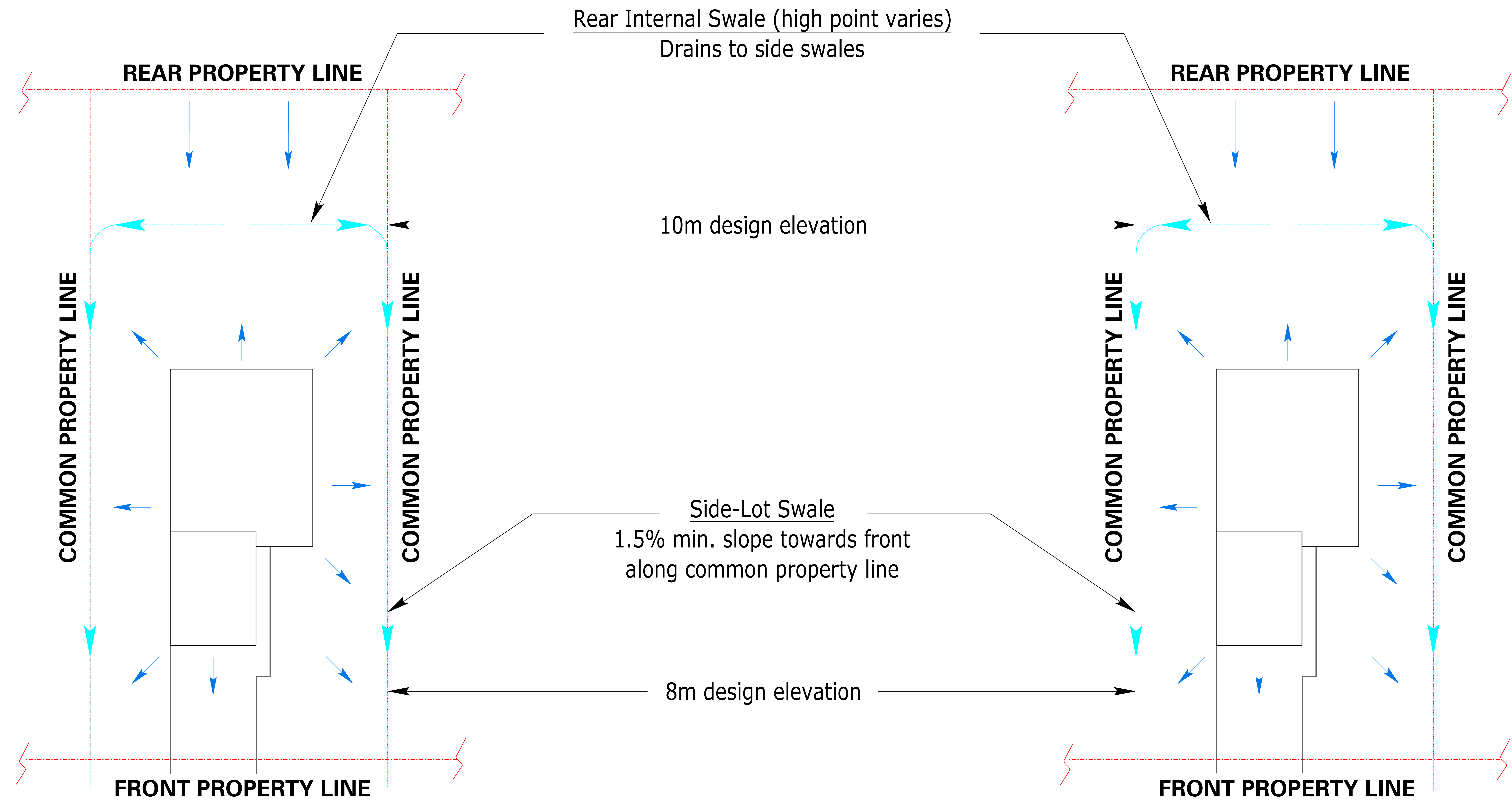
SINGLE-FAMILY RESIDENTIAL LOT TYPE A Rear to front surface drainage with 2-3% overall slope
