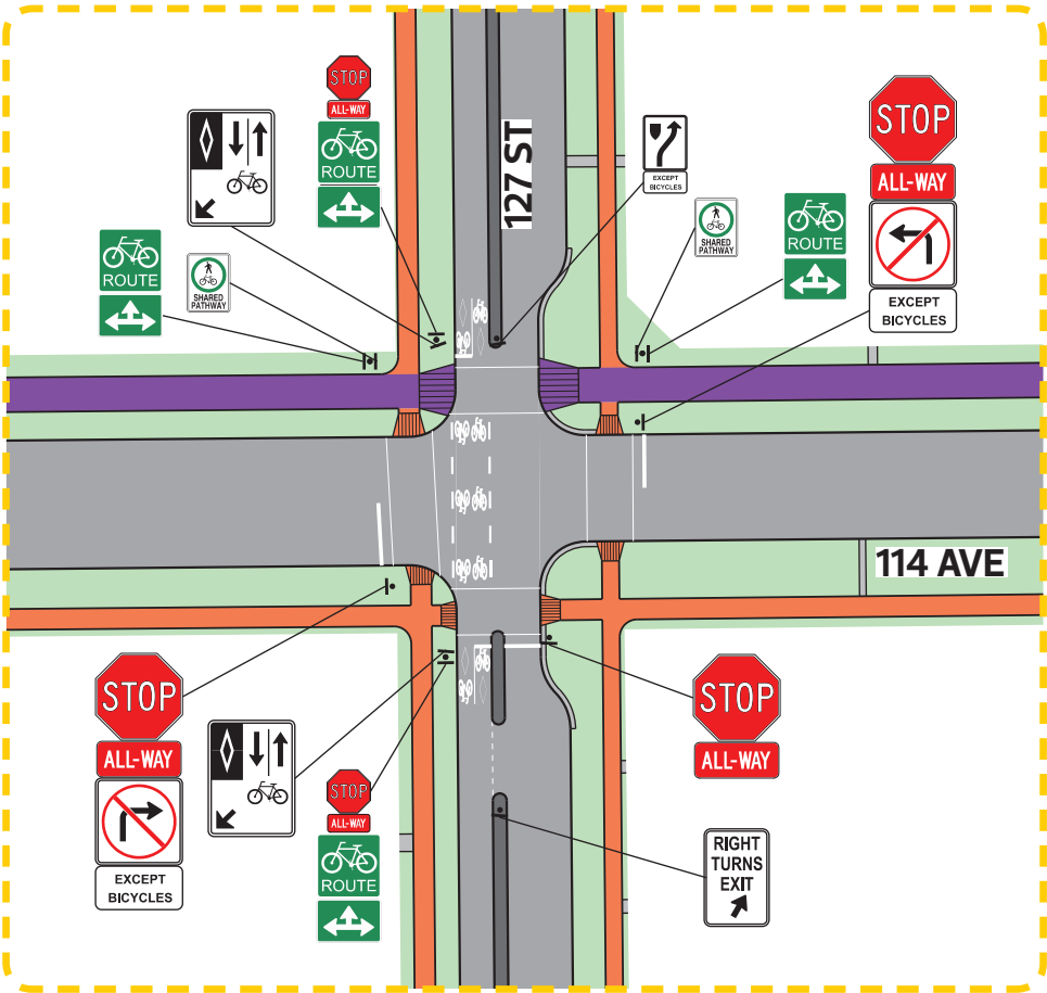
Example Intersection Signage Layout
