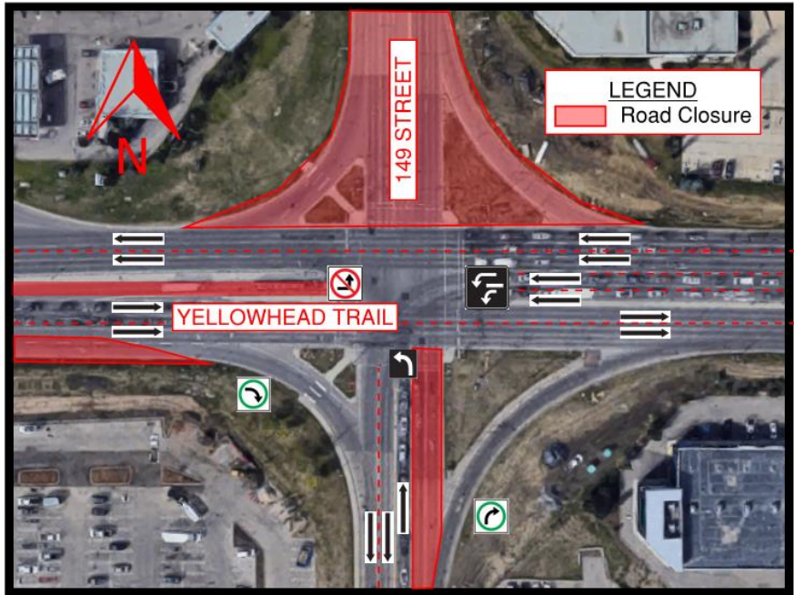
Yellowhead Trail & 149 St - Current Layout
