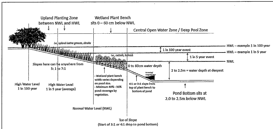
Proposed constructed wetland cross-section (Source: Native Plan Solutions)
