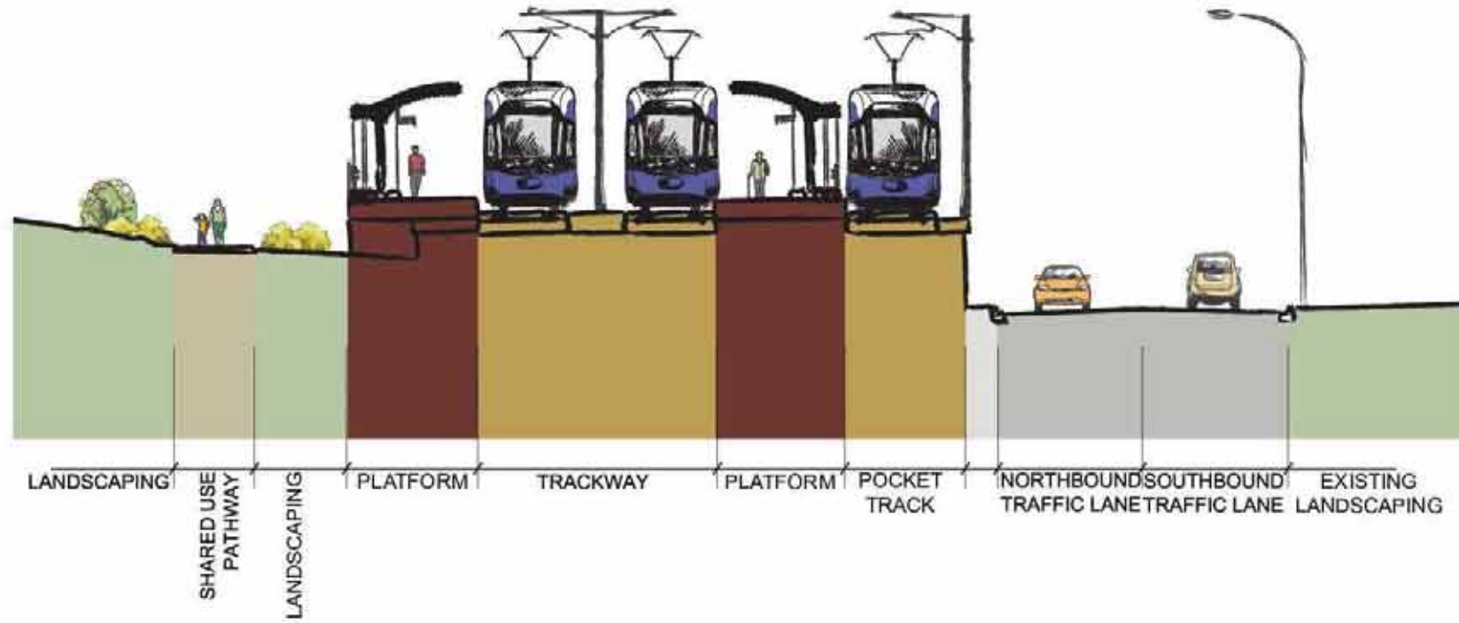
Cross Section A (Looking southwest)
