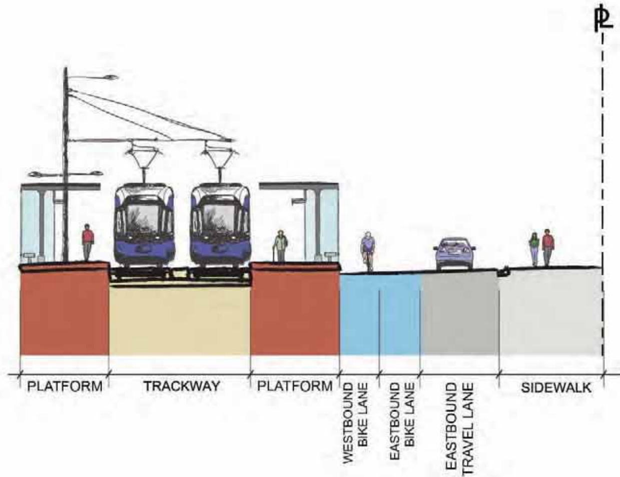
Cross Section B (Looking east)
